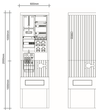
600mm x 1000mm (+1000mm Sockel) x 280mm
